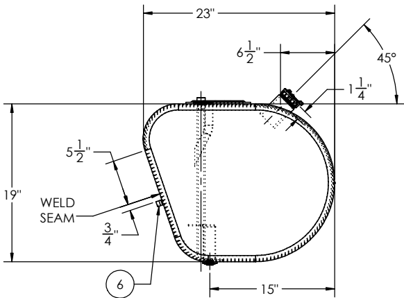
VIEWED FROM LEFT END OF TANK
